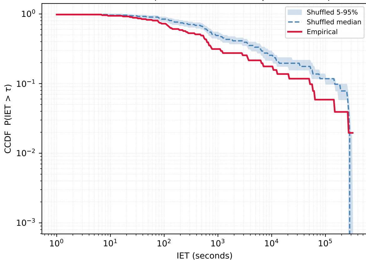
User 1669337139 - Empirical vs Reshuffled | KS=0.223 p=0.000
